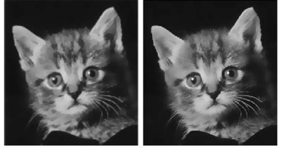
Fig. 2. Edge-preserving smoothing: anisotropic diffusion with 20 time-steps of \tau = 1.0 (left) and Gaussian bilateral filtering with a 15 \times 15 window size, \sigma_D = 5.0 and \sigma_R = 30.0 (right). \sigma_D and \sigma_R are bilateral filtering parameters, see [9] for details.
